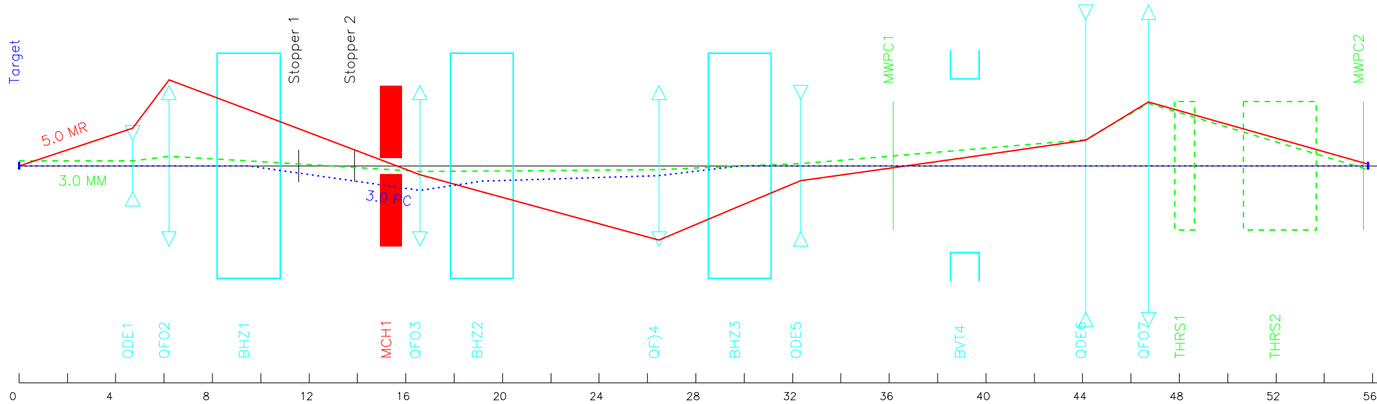
T9 test beam optics
