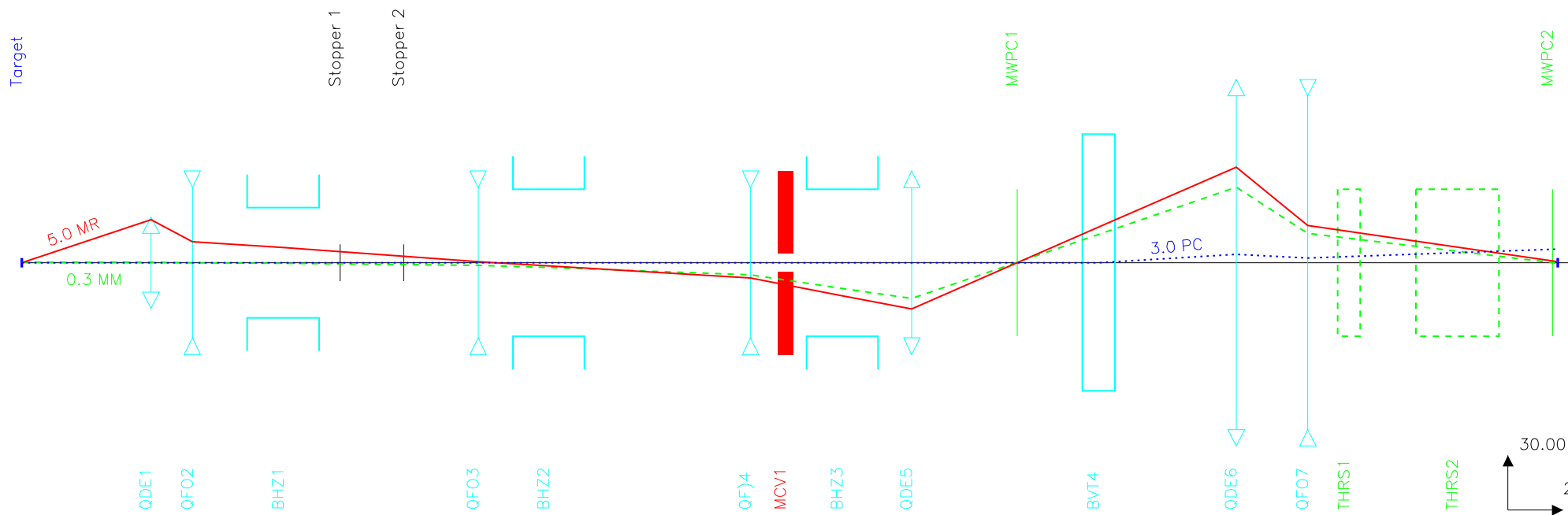
T9 test beam optics
