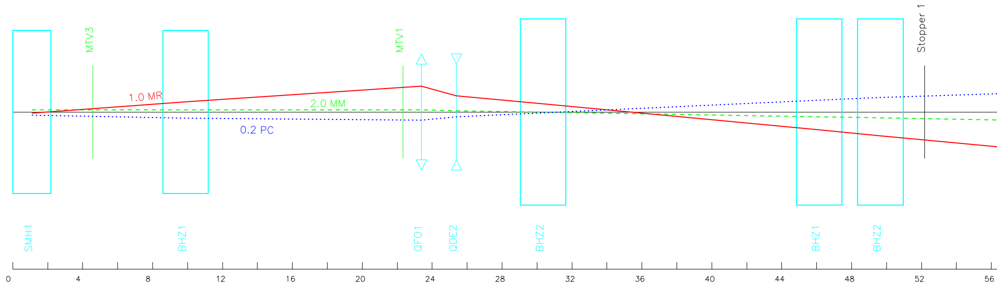
Line T8 for DIRAC
