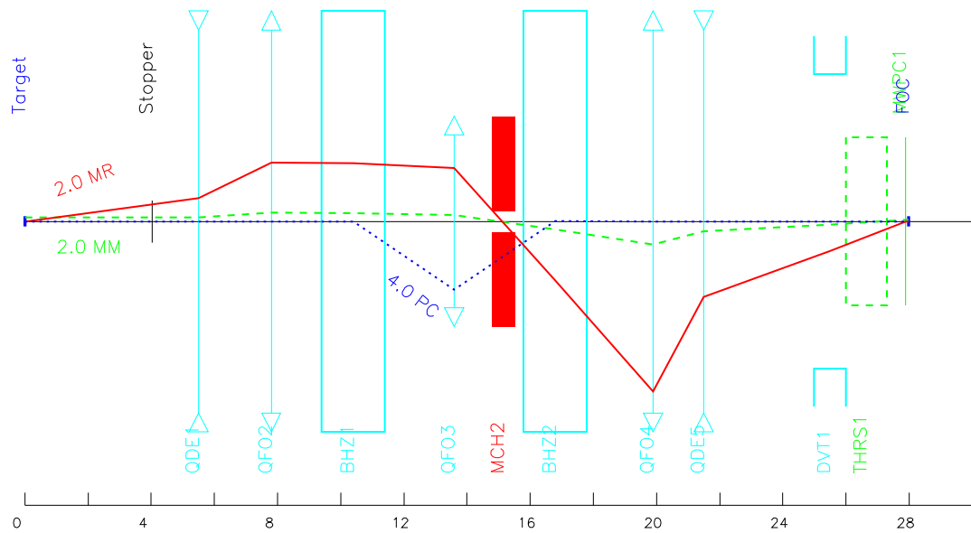
T11 optics – 2006 version
