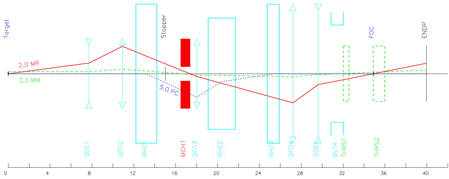
T10 test beam optics
