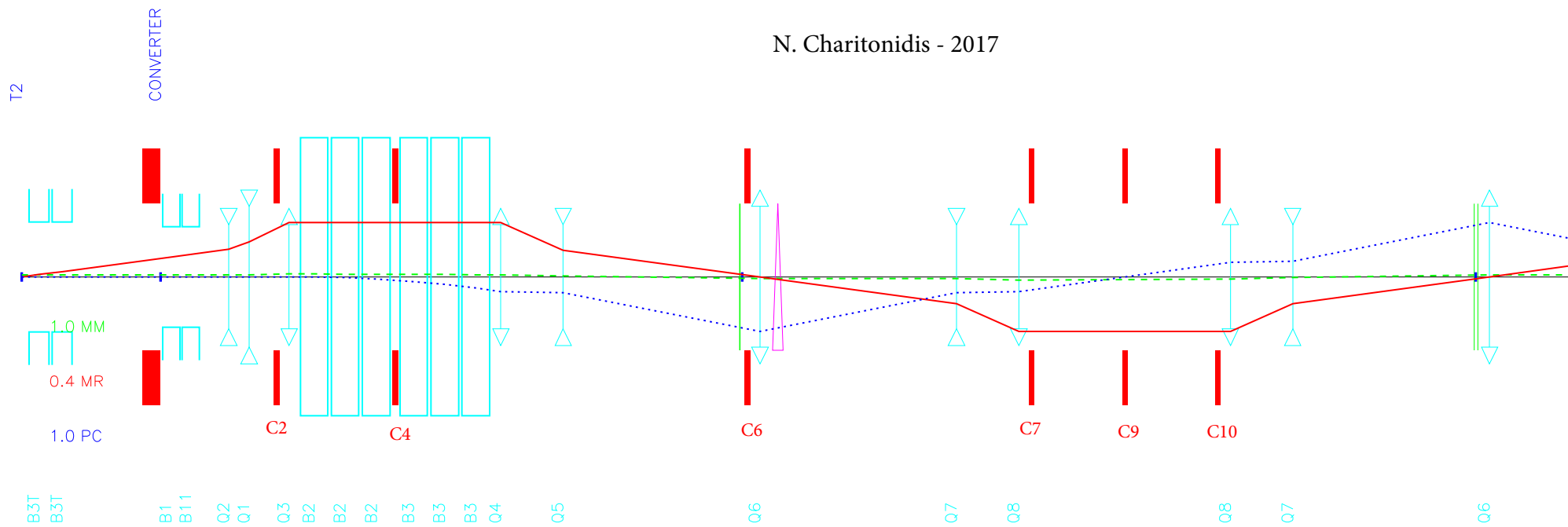
H2 Filter Mode Optics - Focus @ PPE172
